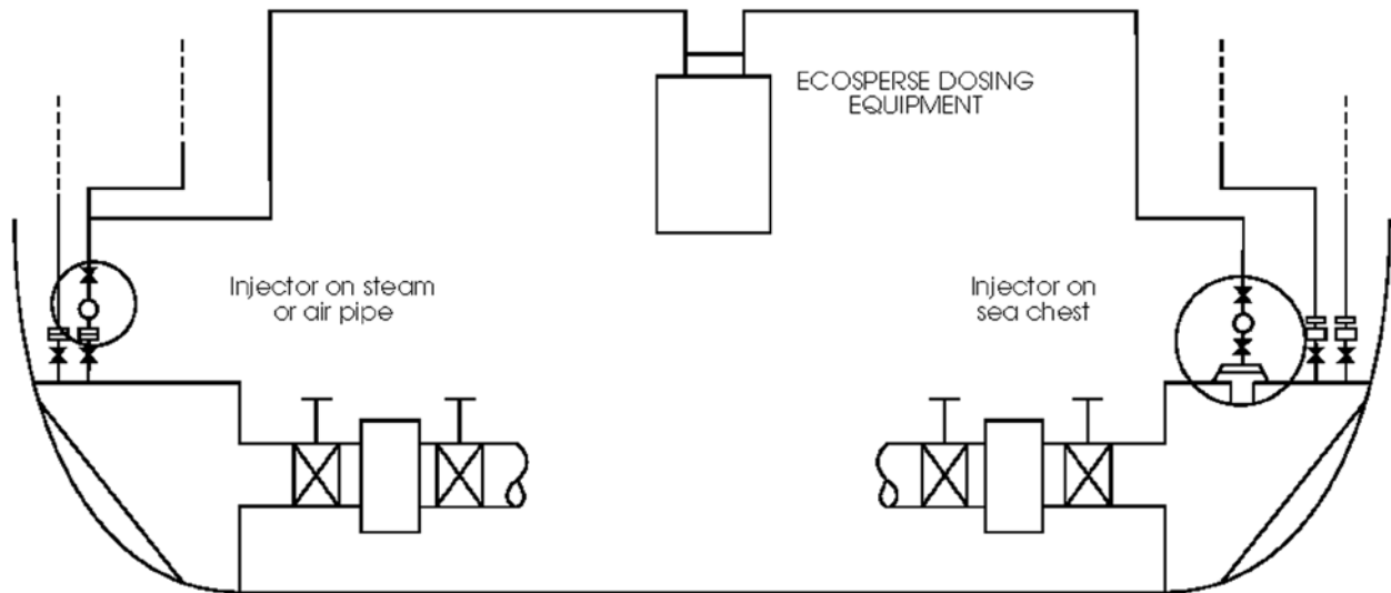
Typical installation of ECOSPERSE dosing equipment Injection point can be fitted also in the sea-chest strainer box
